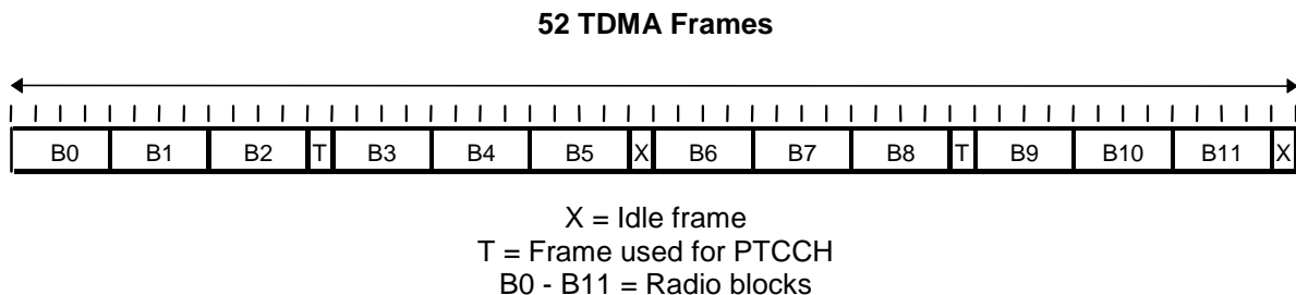
Figure 2a1: 52- multiframe for PDCH/Fs
