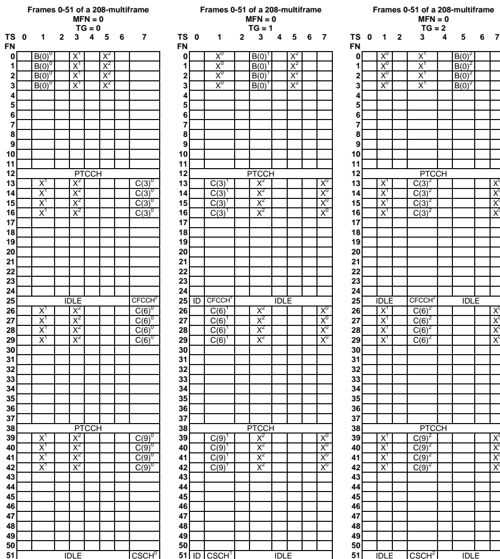
Figure D.2: COMPACT downlink 52-multiframe structure using 3 time groups for nominal cells (based on an assignment of 1 CPBCCH and 3 CPCCCHs with NIB_CCCH_0 = NIB_CCCH_1 = NIB_CCCH_2 = 4, NIB_CCCH_3 = 0). NIB_CCCHs not broadcast for serving cell time group
