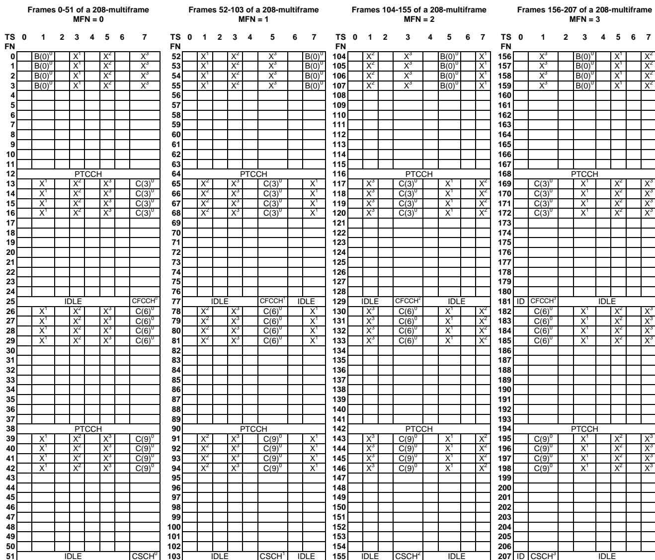
Figure D.5: Example of COMPACT downlink timeslot mapping and rotation of control channels using 4 time groups for nominal cells (based on an assignment of 1 CPBCCCH and 3 CPCCCHs with NIB_CCCH_0 = NIB_CCCH_1 = NIB_CCCH_2 = NIB_CCCH_3 = 4). TG = 0 is illustrated. NIB_CCCH is not broadcast for serving cell time group
