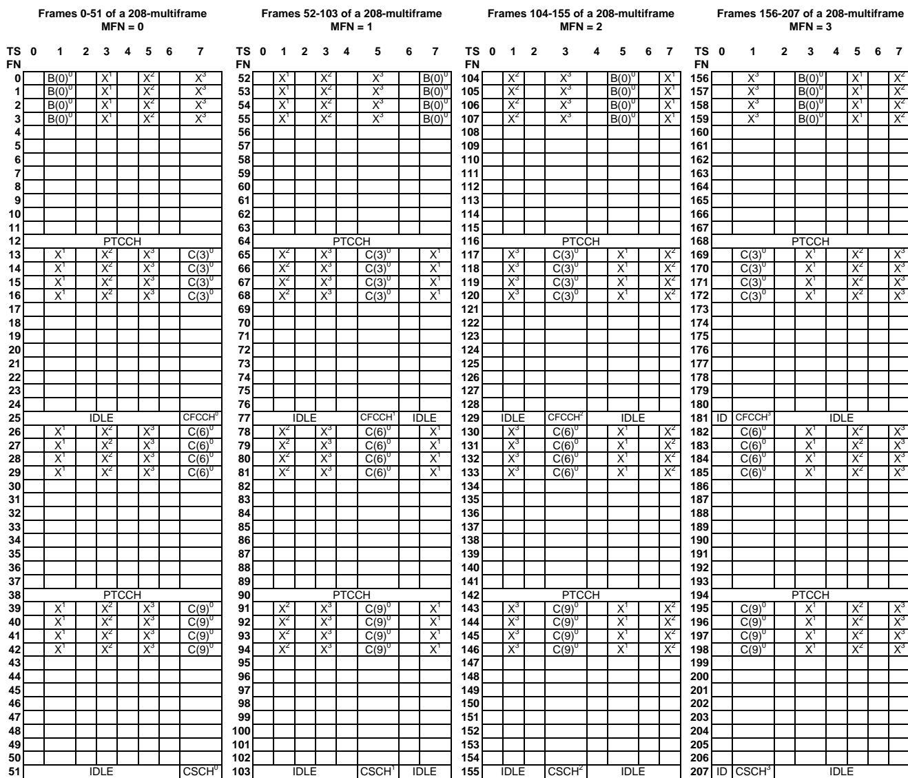
Figure D.5: Example of COMPACT downlink timeslot mapping and rotation of control channels using 4 time groups for nominal cells (based on an assignment of 1 CPBCC and 3 CPCCs with NIB_CCCH_0 = NIB_CCCH_1 = NIB_CCCH_2 = NIB_CCCH_3 = 4). TG = 0 is illustrated. NIB_CCCH is not broadcast for serving cell time group
