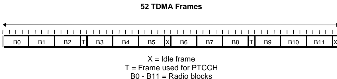
Figure 9: 52- multiframe for PDCHs -
