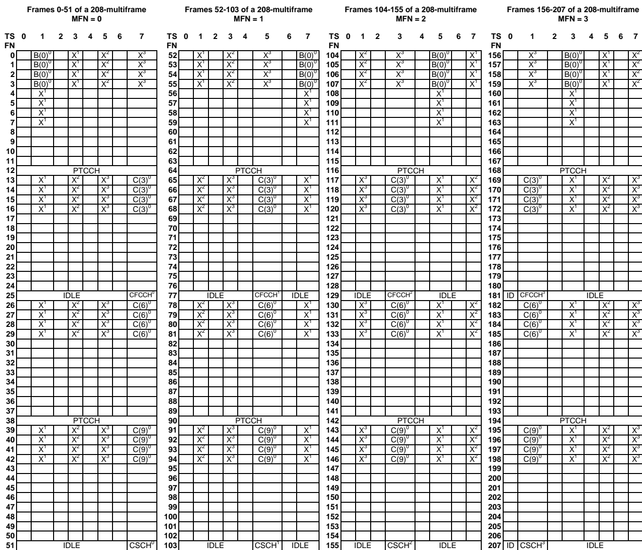
Figure D.7: Example of COMPACT downlink timeslot mapping and rotation of control channels using 4 time groups for nominal cells (based on an assignment of 1 CPBCCH and 3 CPCCCHs with NIB_CCCH_0 = NIB_CCCH_2 = NIB_CCCH_3 = 4, NIB_CCCH_1 = 5). TG = 0 is illustrated. NIB_CCCH is not broadcast for serving cell time group
