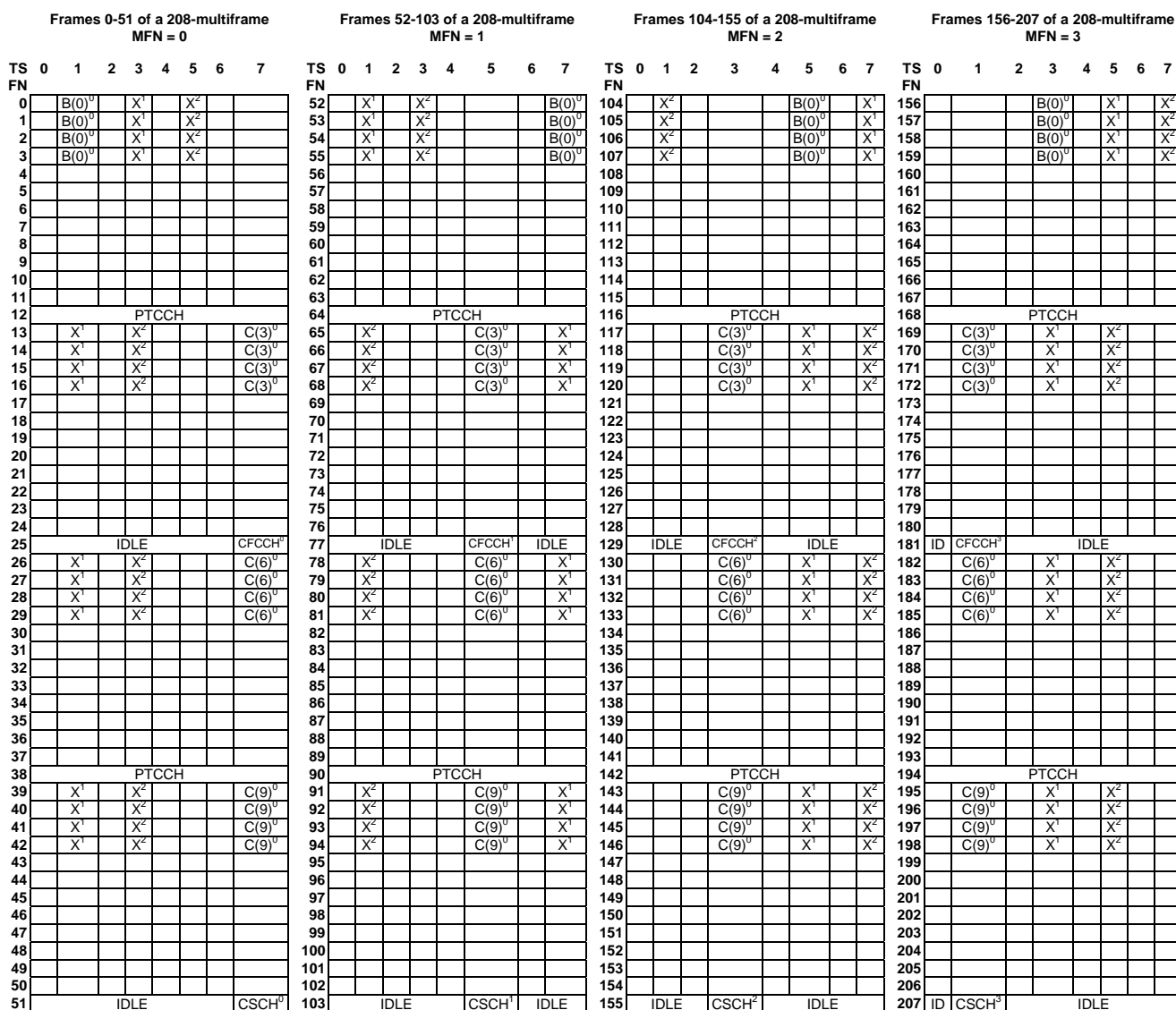
Figure D.6: Example of COMPACT downlink timeslot mapping and rotation of control channels using 3 time groups for nominal cells (based on an assignment of 1 CPBCC and 3 CPCCs with NIB_CCCH_0 = NIB_CCCH_1 = NIB_CCCH_2 = 4, NIB_CCCH_3 = 0). TG = 0 is illustrated. NIB_CCCH is not broadcast for serving cell time group
