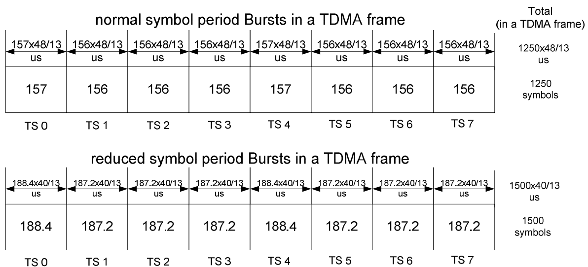
Figure 5.7.1: Implementation allowing integral number of symbol periods for normal symbol period bursts.
