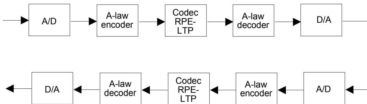
Figure A.1.2: Two - transcodings scheme (A-law)
