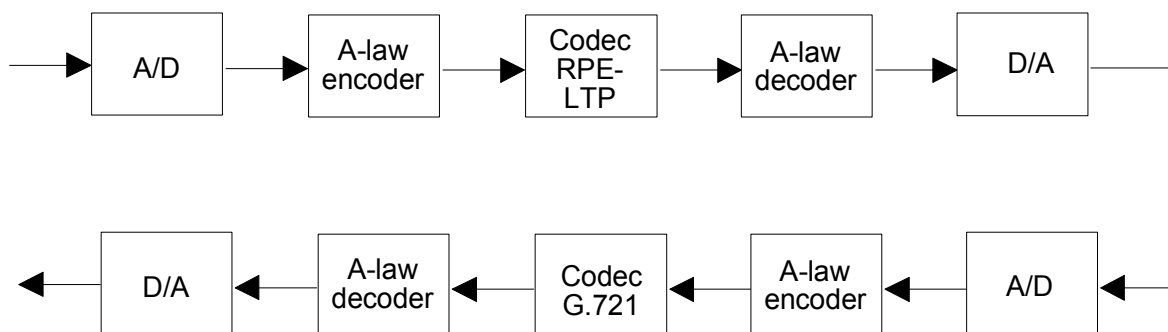
Figure A.1.3: Mixed transcodings - scheme 1 (A-law)
