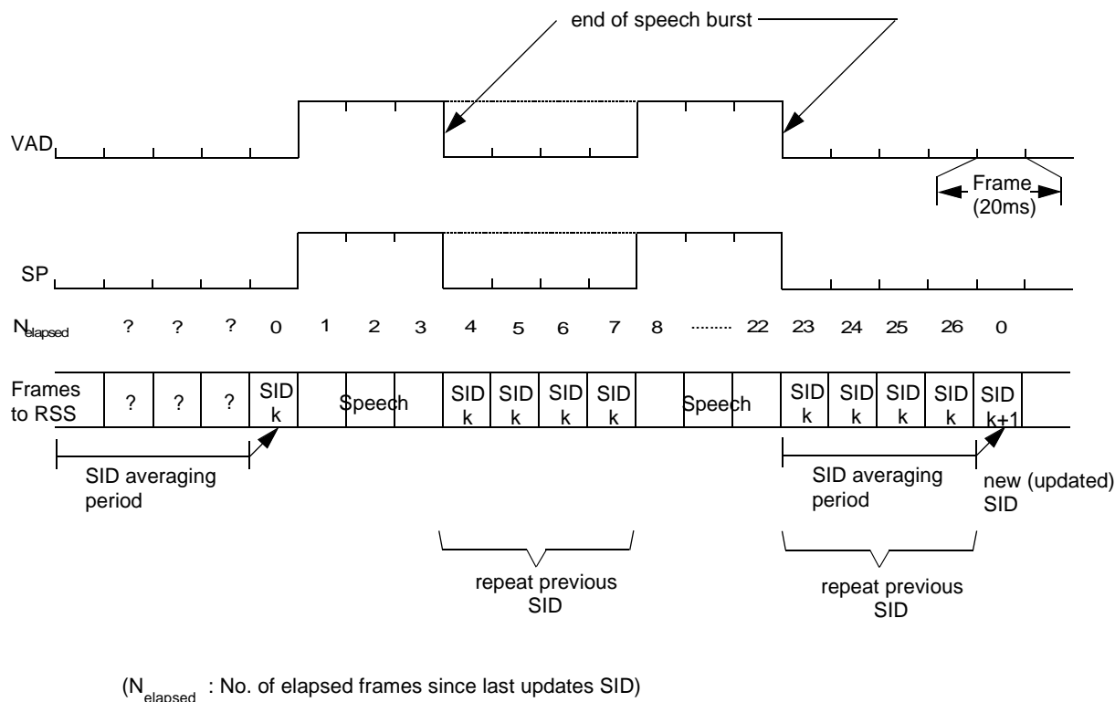
Figure 3: Handling of short speech bursts ( N_{elapsed} < 24 ) (Example)
