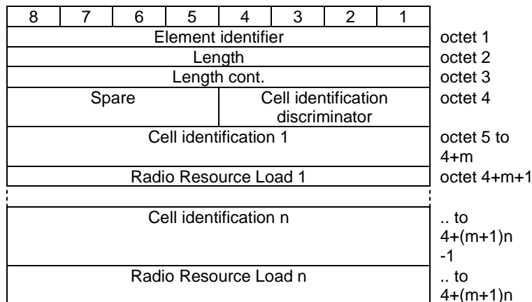
Figure 8.2.12.1: Radio Resource Loading List information element
