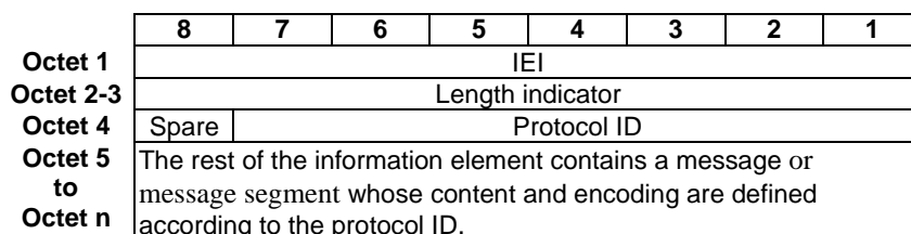
Figure 10.3.1: APDU IE
