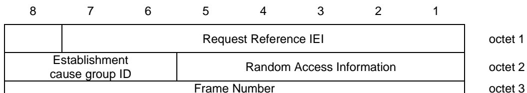
Figure 11.15: request reference IE
