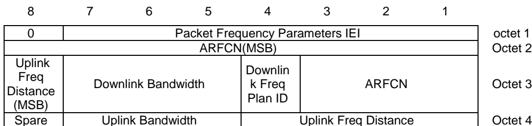
Figure 11.51.4: Packet Frequency Parameters IE
