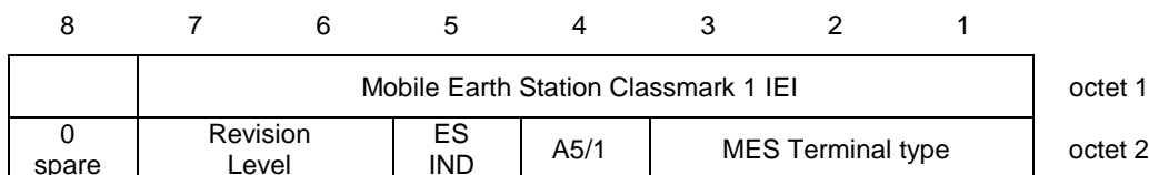
Figure 11.3: Mobile Earth Station classmark 1 IE
