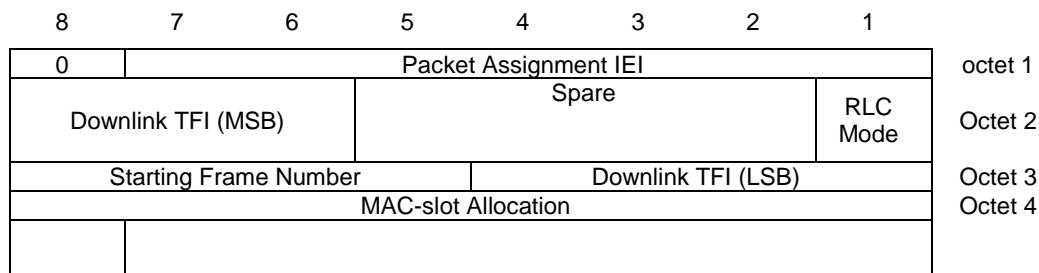
Figure 11.51.3: Packet Immediate Assignment Type 3 Parameters IE
