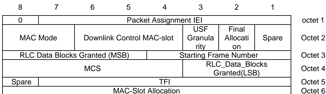
Figure 11.51.5: Packet Immediate Assignment Type 2 Parameters IE
