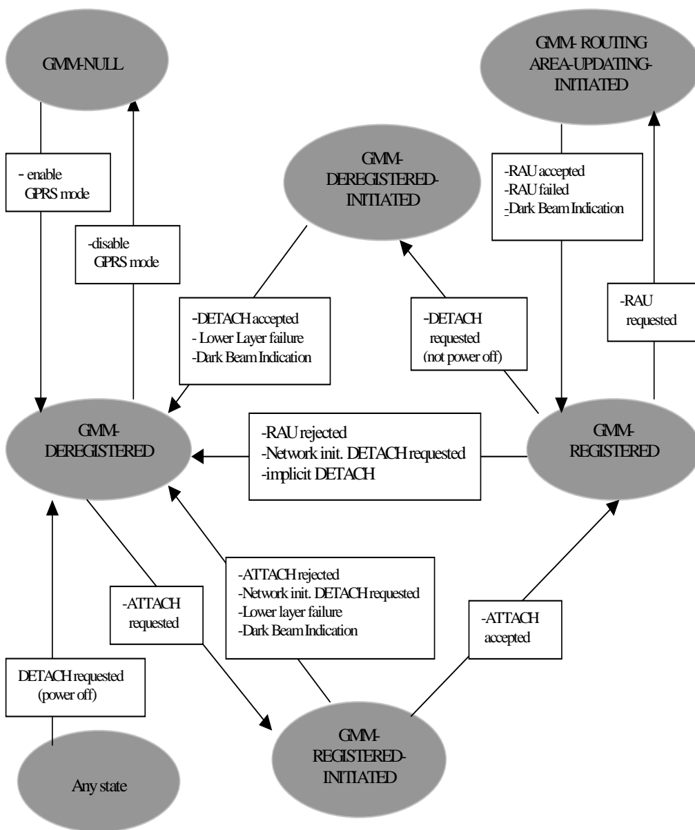
Figure 5.1b: GMR-1 04.008: GMM main states on the MES side
