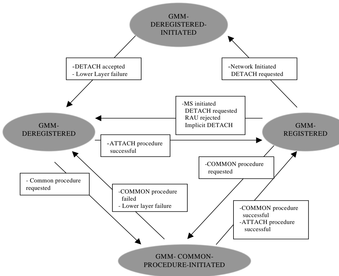
Figure 5.1c: GMR-1 04.008: GMM main states on the network side
