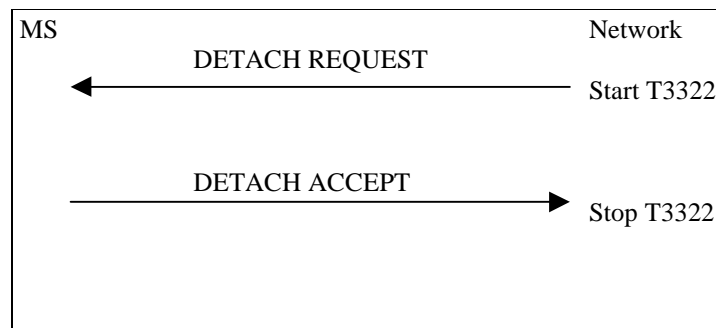
Figure 5.7.4: 2 GMR-1 04.008: Network initiated GPRS detach procedure
