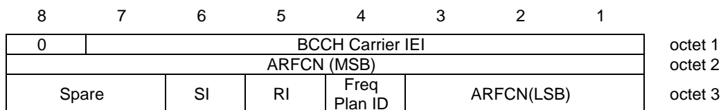
Figure 11.51.2: Packet BCCH carrier IE
