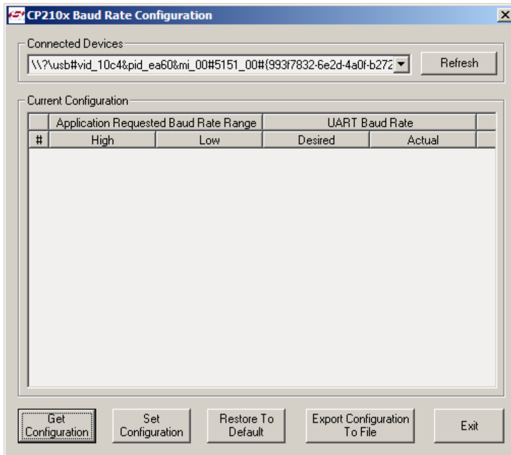
Figure 1. Main Window
