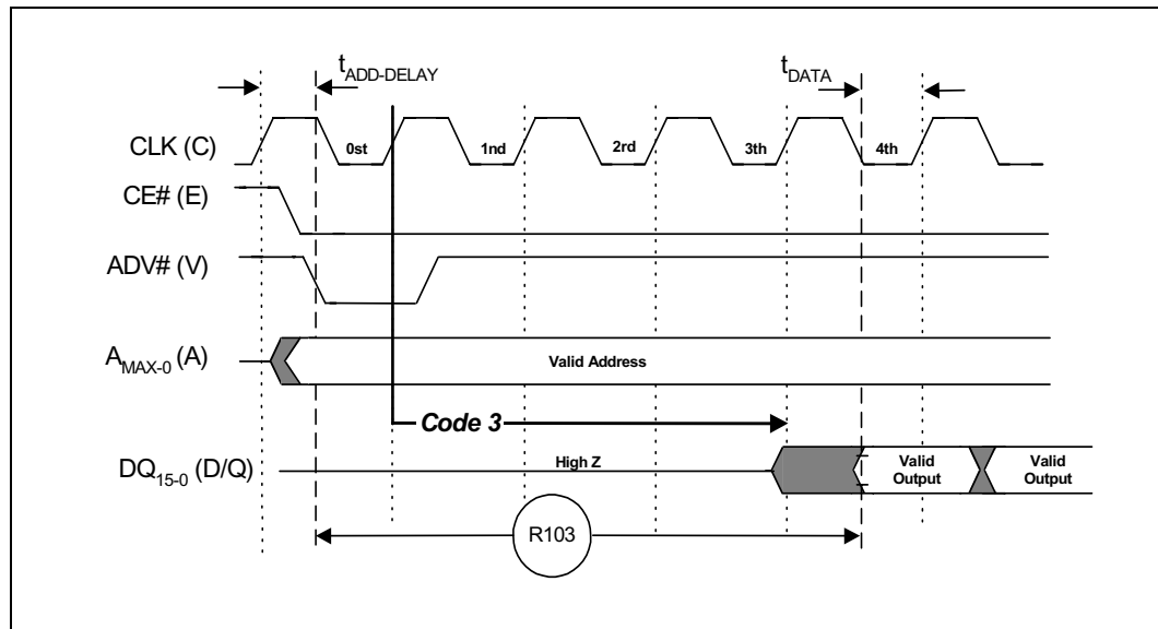
Figure 18. Data Output with LC Setting at Code 3
