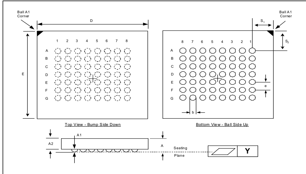
Figure 41. 32-, 64- and 128-Mbit VF BGA CSP Package Drawing
