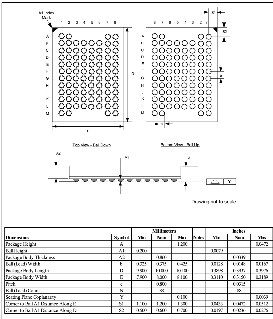
Figure 42. 64Mbit and 128Mbit QUAD+ Package Drawing
