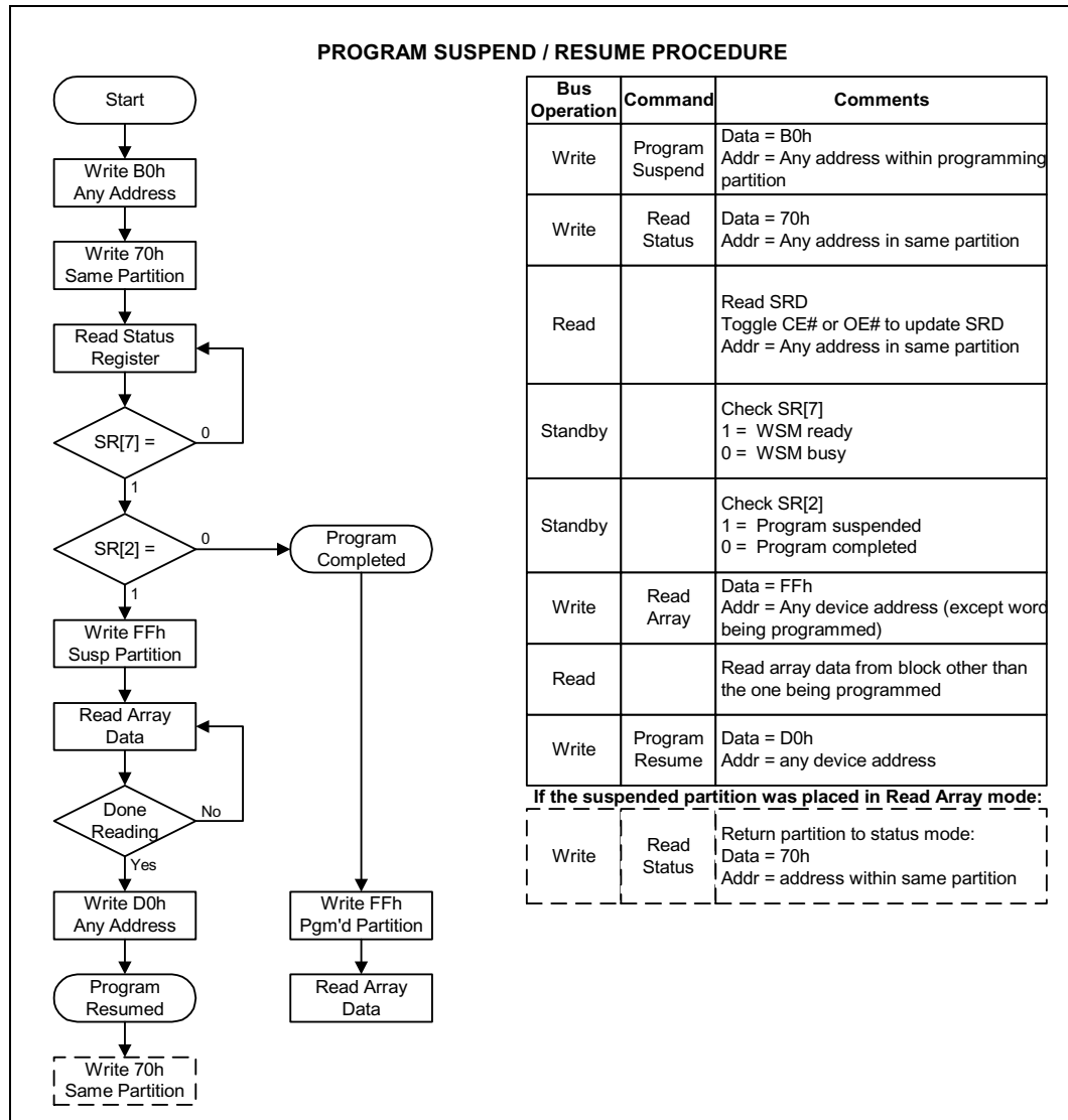
Figure 8. Program Suspend / Resume Flowchart
