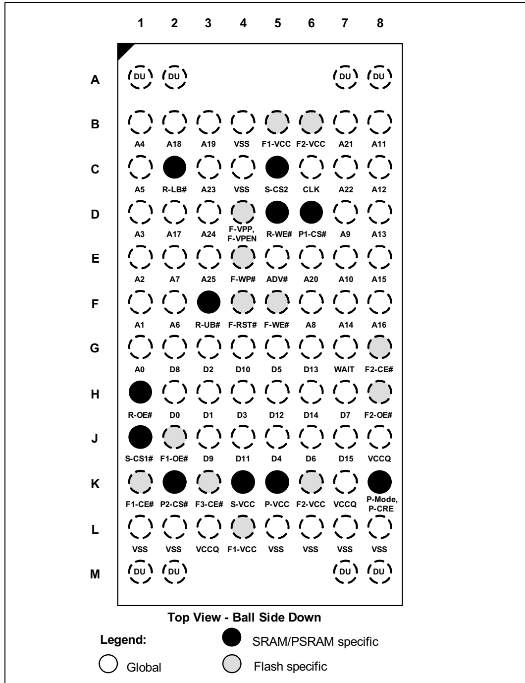
Figure 2. 88-Ball (80 active balls) QUAD+ Ballout
