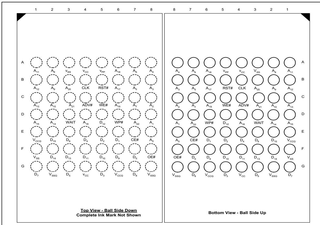
Figure 1. 56-Ball VF BGA/ \mu BGA Ballout
