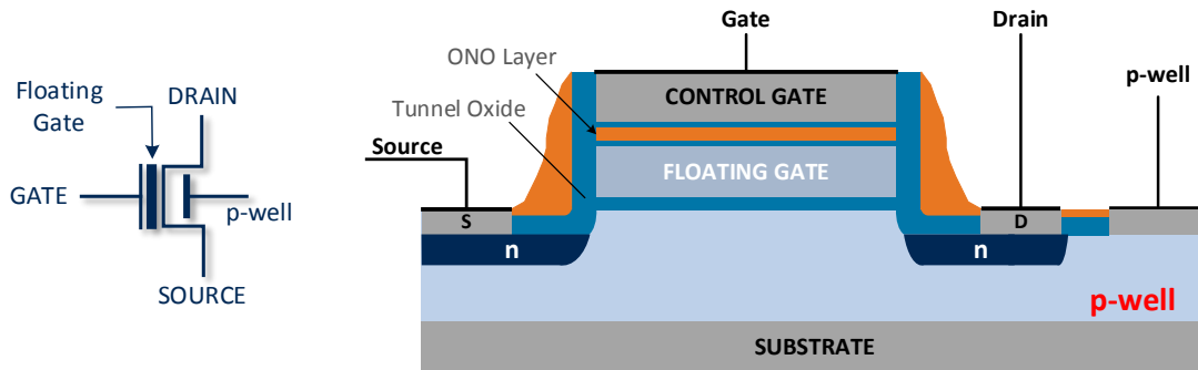
Figure 1 Symbol and structure of a floating gate MOSFET
