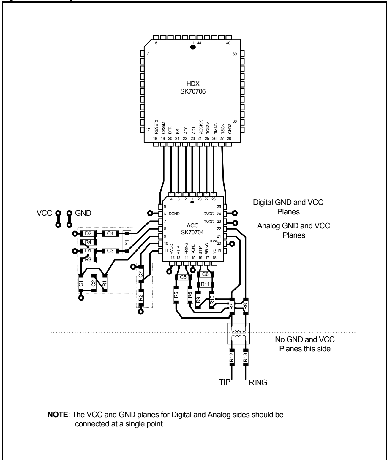
Figure 11: PCB Layout Guidelines
